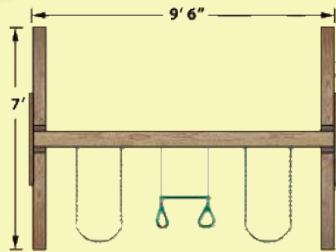
3 POSITION A-FRAME INCLUDES 2 BELT SWINGS & 1 TRAPEZE BAR
