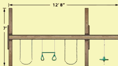
3XP EXTENDED BEAM A-FRAME INCLUDES 2 BELT SWINGS, 1 TRAPEZE BAR & 1 DISK SWING
