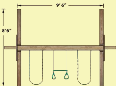
INCREASING BEAM HEIGHT OFFERS HIGHER SWING ARC
