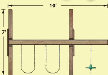
2XP EXTENDED BEAM A-FRAME INCLUDES 2 BELT SWINGS & 1 DISK SWING
